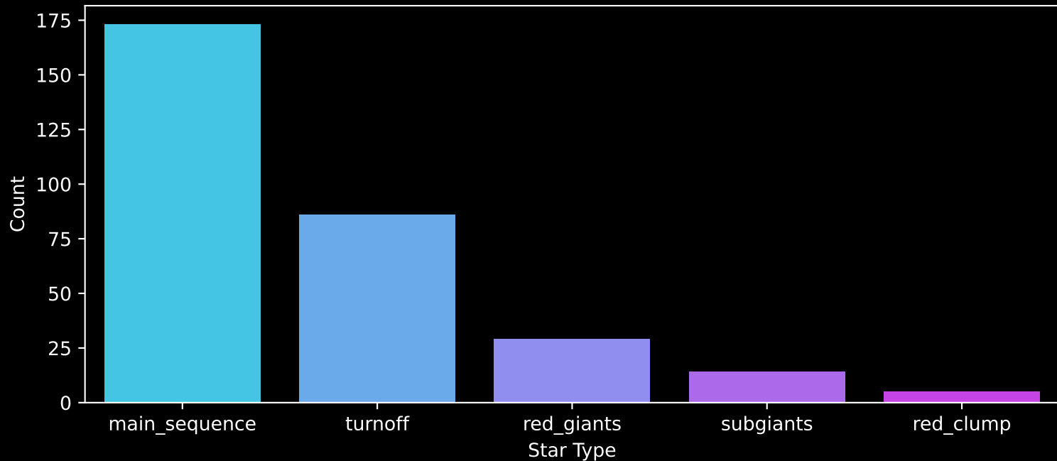
GALAH DR4 Field: [201] Count plot of Star Type
