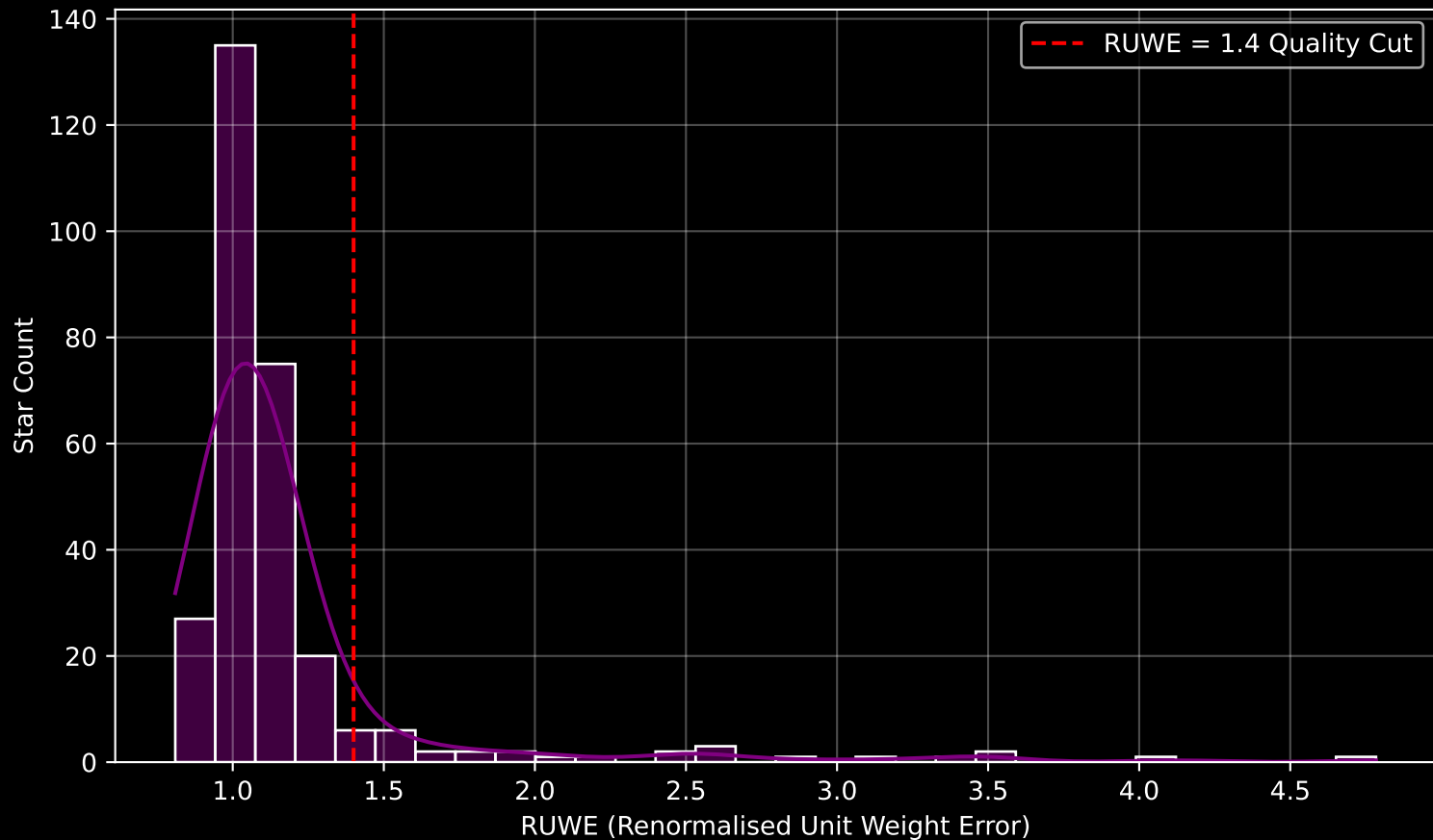
GALAH DR4 Field [201] RUWE Distribution (n= 289)
