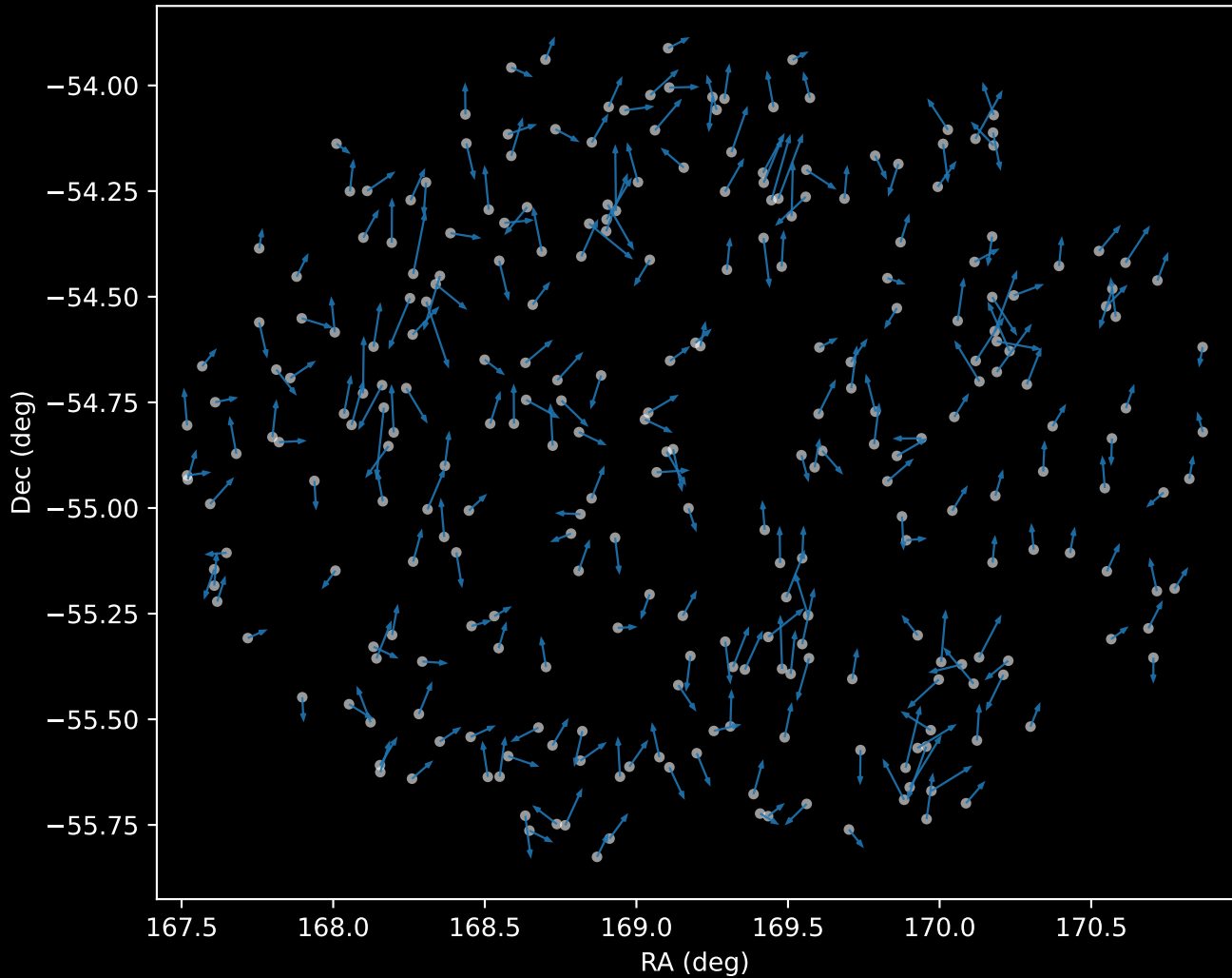
GALAH DR4 Cluster 0 Proper Motion Vectors (n=273)
